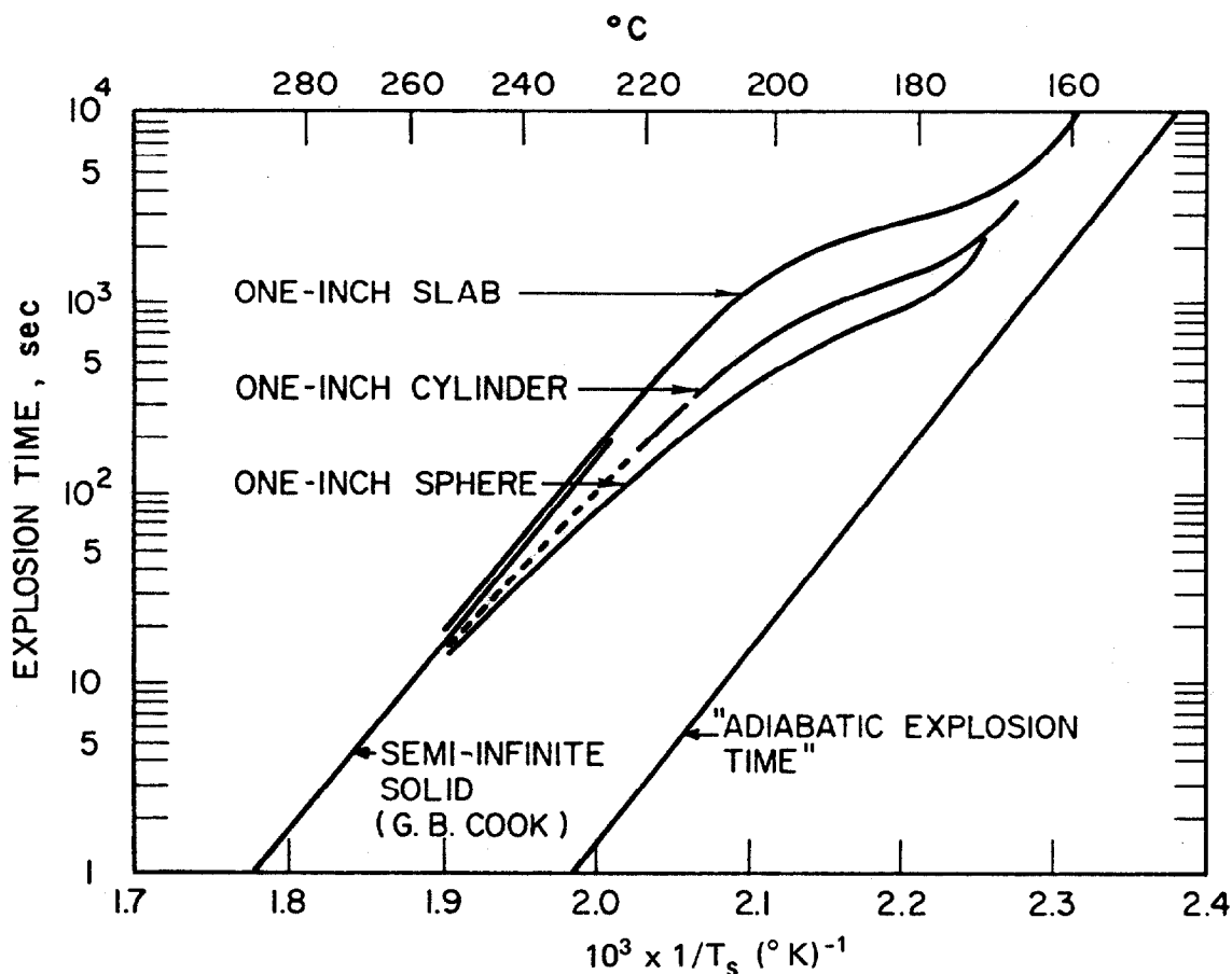
Fig 5 Explosion Times vs 1/T_s for RDX in Various Geometries, Initially at 25^\circ\text{C} (Ref 6)
